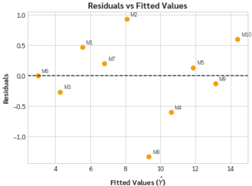
Figure 3 (Residuals vs Fitted): Residuals vs. Fitted plot to check for non-linear patterns and homoscedasticity. Points scattered randomly around the 0 line indicate a good fit.
