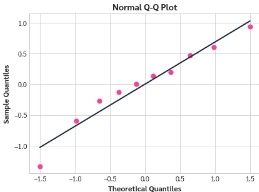
Figure 5 (Q-Q Plot): Q-Q plot comparing the quantiles of the residuals against a standard normal distribution. Points closely following the diagonal line suggest normality.
