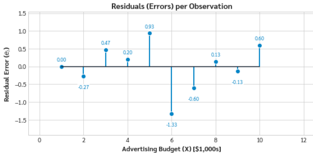
Figure 2 (Residuals Lollipop Plot): Lollipop plot illustrating the residuals for each observation, showing the vertical distance between actual and predicted sales.
