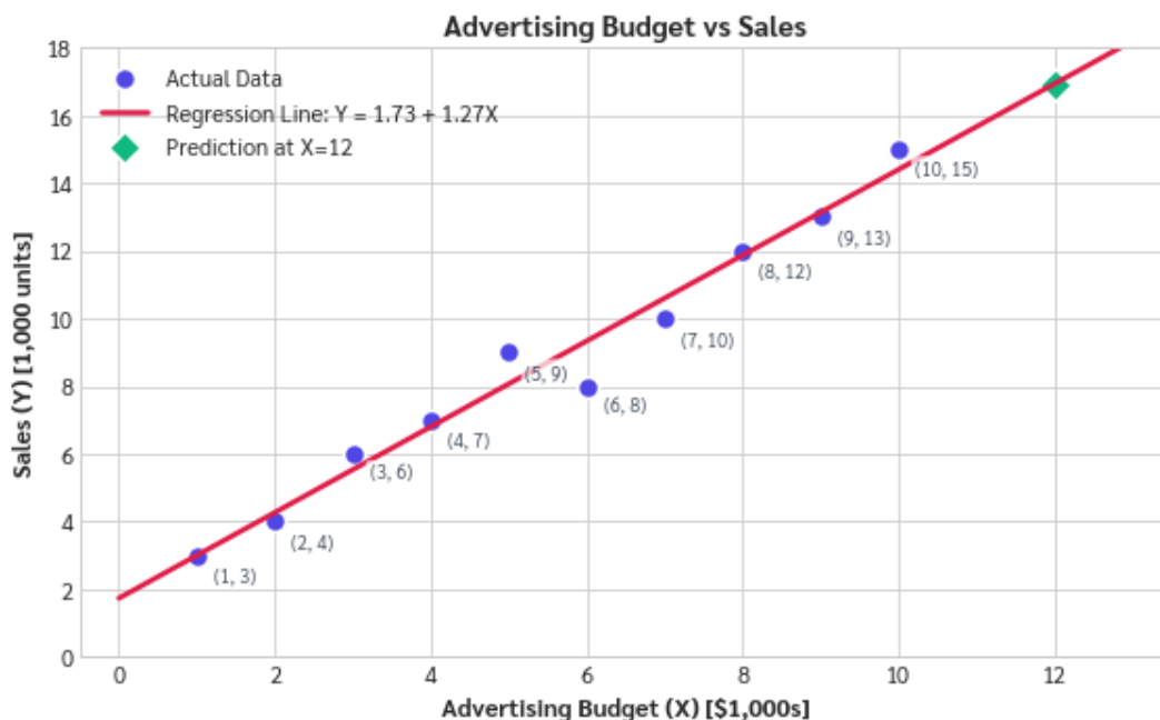
Figure 1 (Regression Line): Scatter plot displaying the relationship between Advertising Budget and Sales, with the fitted OLS regression line.
