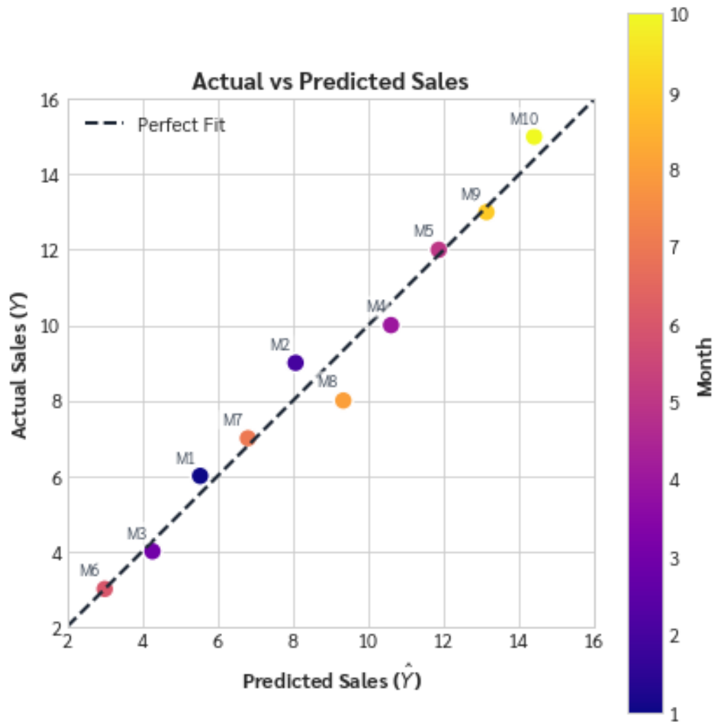
Figure 7 (Actual vs Predicted): Actual vs. Predicted values plot to visualize the overall fit of the model. Points close to the diagonal dashed line indicate accurate predictions.
