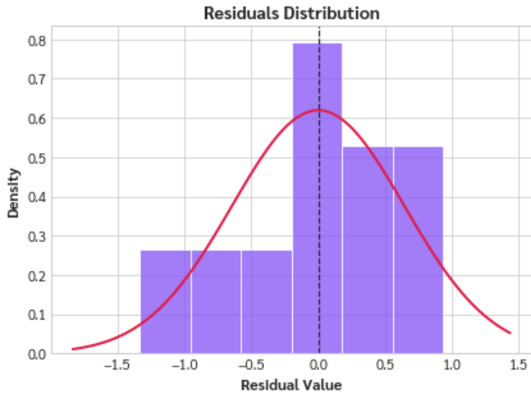
Figure 4 (Residuals Distribution): Histogram of residuals to assess whether they approximate a normal distribution (Normality assumption).
