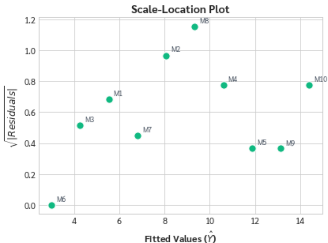
Figure 6 (Scale-Location): Scale-Location plot to check for homoscedasticity (equal variance of residuals) across the range of fitted values. The trend line should be relatively horizontal.
